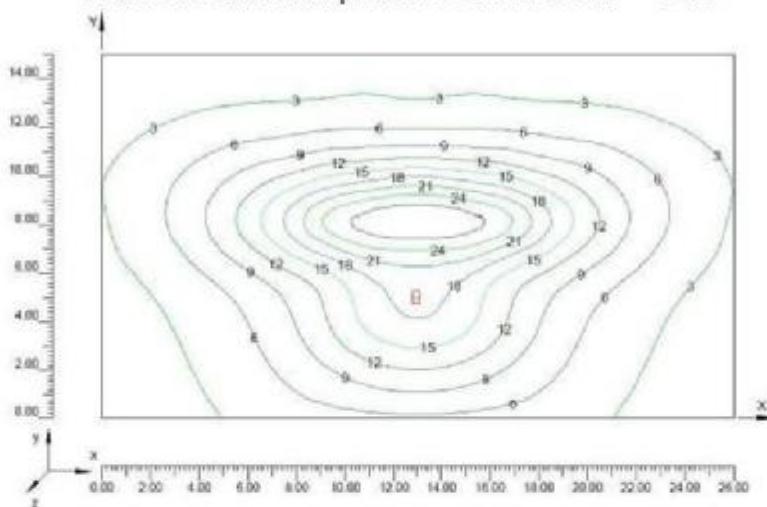
Curve isolux lampada SOX-E 36 h = 6 m
