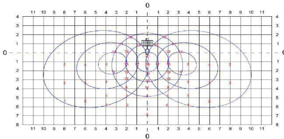
Curve ISOLUX Lampada 20 led h = 6.00 m
