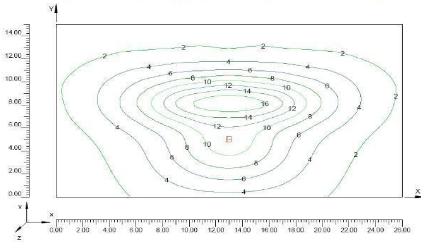
Curve isolux lampada SOX-E 26 h = 6 m
