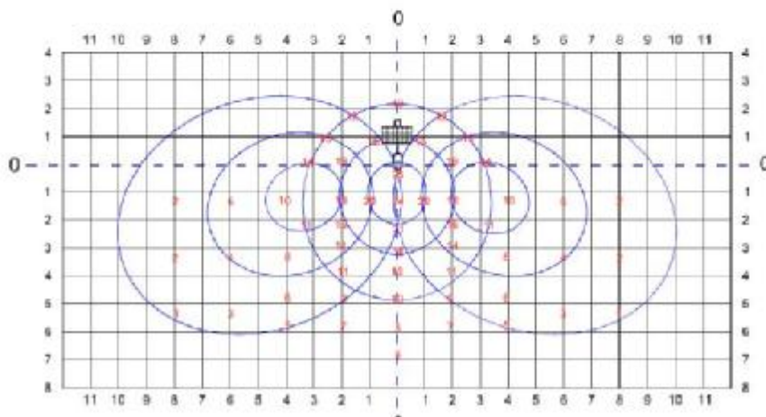
Curve ISOLUX Lampada 24 led h = 6.00 m
