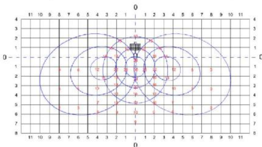
Curve ISOLUX Lampada 30 led h = 6.00 m
