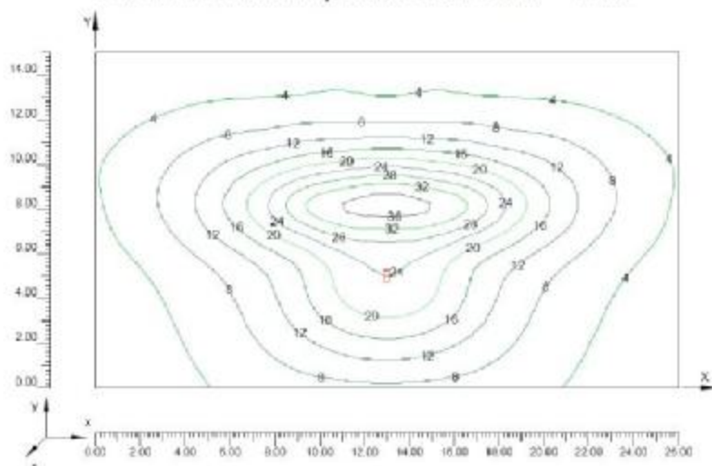
Curve ISOLUX Lampada 30 led h = 6.00 m
